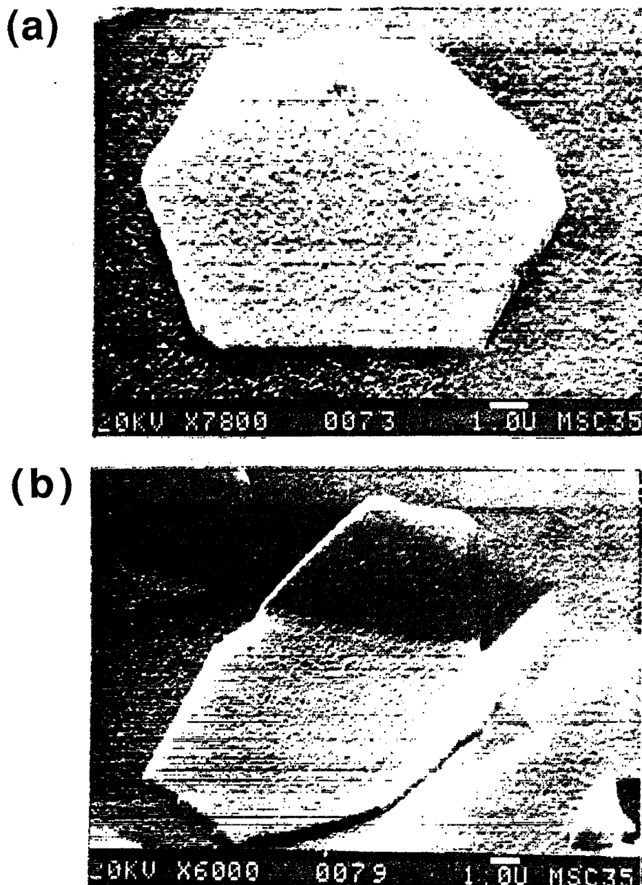
FIG. 3. SEM micrograph of Si crystals on polysilicon after Au was selectively etched. Au( \approx 250 nm)/polysilicon( \approx 400 nm)/SiO 2 samples were fabricated on (a) flat and (b) stepped-surface substrates.
