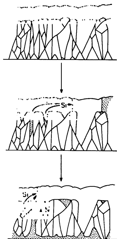
FIG. 10. Stages of grain growth of Si crystals. The initial structure is a bilayer of Au (top) and of polysilicon with various grain sizes (bottom). Note that the resultant large-grained crystal has the same orientation as the initial grain.
